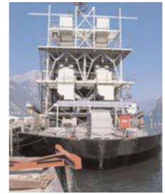
Front view of the two screening plants
