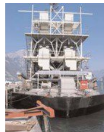
Front view of the two screening plants
